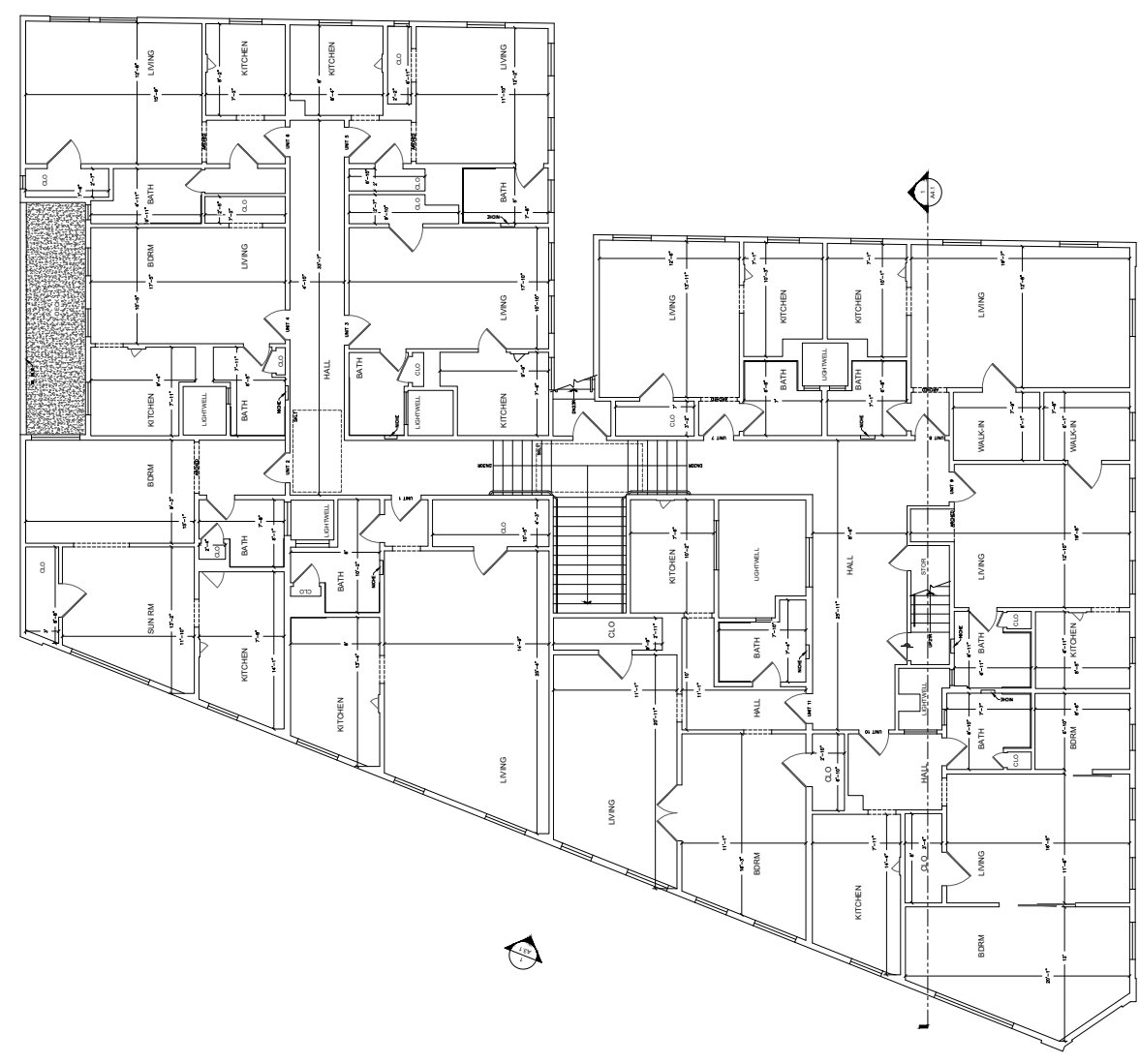
EXISTING UPPER LEVEL FLOOR PLAN 100 CITY AVENUE, 100 100 CITY AVENUE, 100
