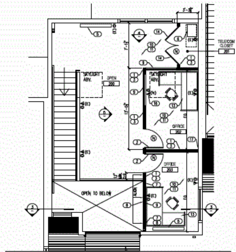
2 2nd Floor - Construction Plan Scale: 1/8" = 1'-0" North
