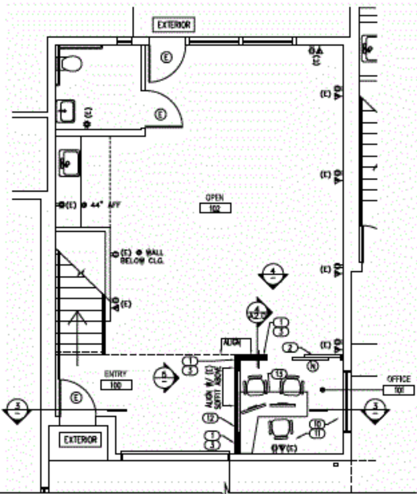
1 Ground Floor - Construction Plan Scale: 1/8" = 1'-0" North
