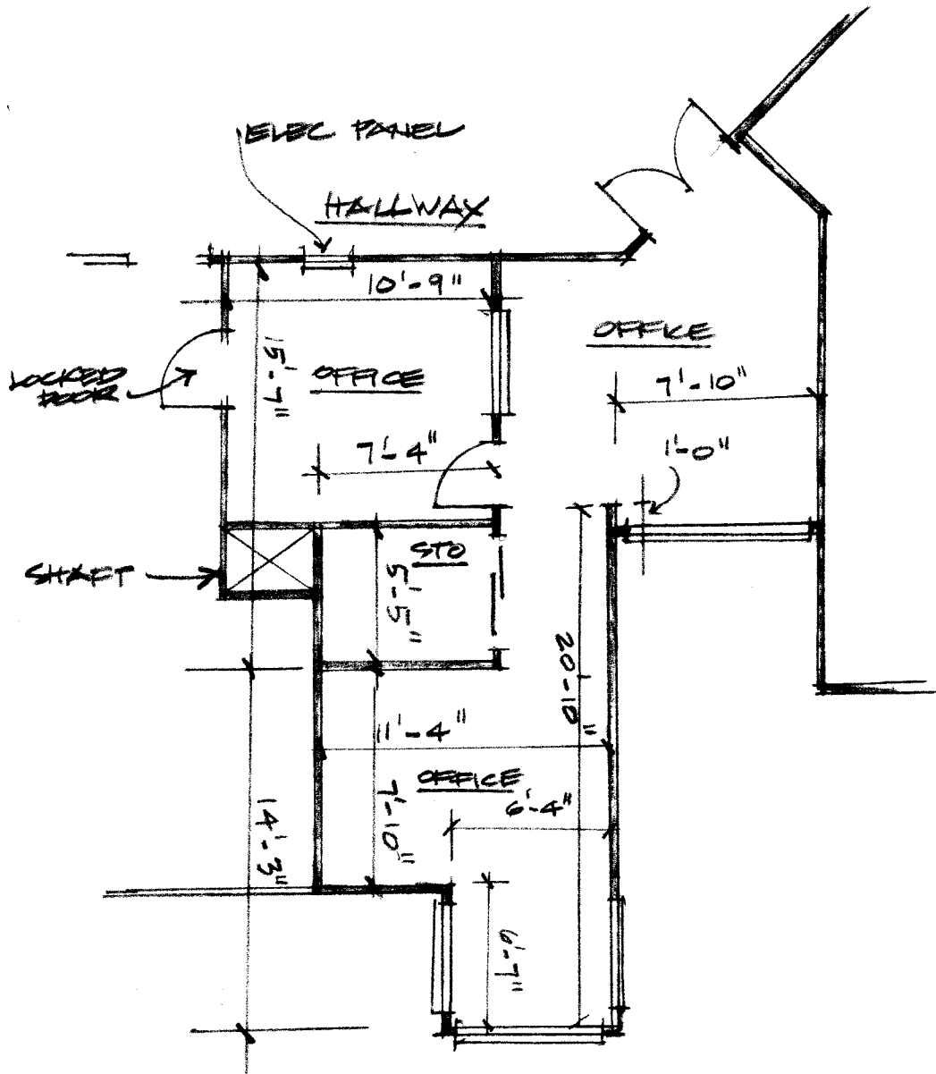
SUITE 9 SKETCH NTS
